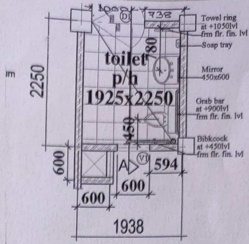
Typical Plan of toilet (P/H)
